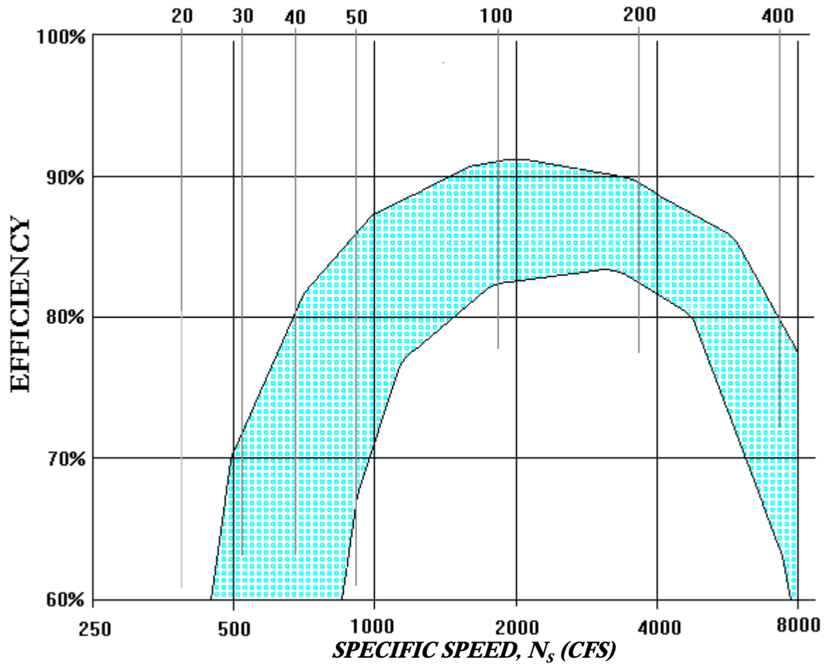
Figure 20-2 Range of Efficiencies
